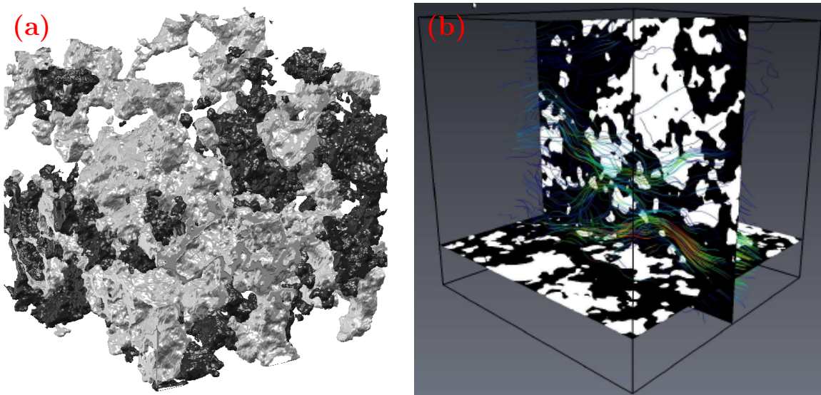
Figure 10: 3D view of the reconstructed model (a) made of GDC (light grey) and LST (dark grey). Pores are transparent. (b) Gaz flow occurring in the porosity of a (model of) GDC10 anode cell layer.
