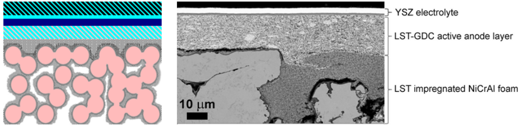
Figure 2: The EVOLVE cell, a metallic foam supported cell.
