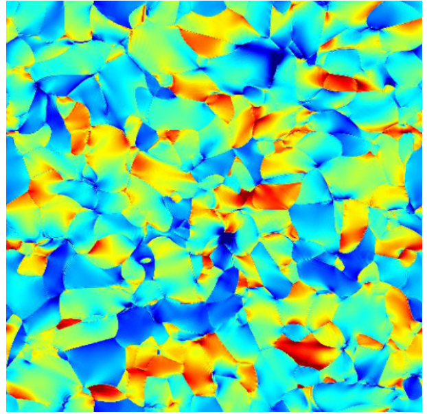
Figure 10: Example of pressure field under applied temperature increase of 1 K and zero strains. Color scale: minimum (red) is -5.1 \text{ MPa or MPa.K}^{-1} , maximum (blue) is -3.6 \text{ MPa or MPa.K}^{-1} .
