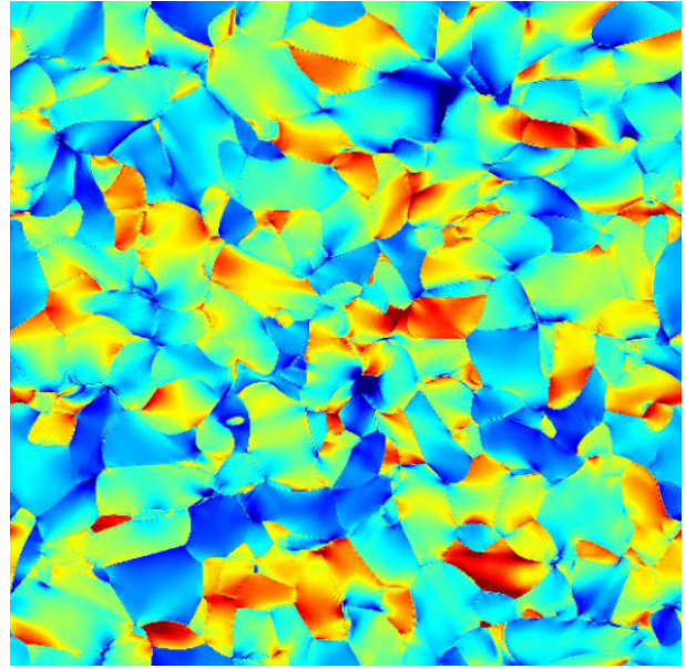
Figure 10: Example of pressure field under applied temperature increase of 1 K and zero strains. Color scale: minimum (red) is -5.1 \text{ MPa or MPa.K}^{-1} , maximum (blue) is -3.6 \text{ MPa or MPa.K}^{-1} .
