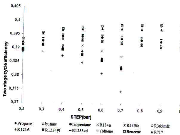
Fig. 3. Two Stage Cycle efficiency calculation results
