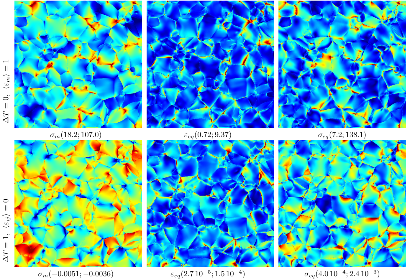
Figure 16: 2D sections of the mean stress \sigma_m , Von Mises equivalent strain \varepsilon_{eq} and stress fields \sigma_{eq} (left to right), with applied hydrostatic strain loading \langle \varepsilon_m \rangle = 1 , \Delta T = 0 (top) and thermal loading \Delta T = 1 , \langle \varepsilon_m \rangle = 0 (bottom). The x axis is oriented top to bottom and the y axis left to right. To highlight the field patterns, the highest and lowest 0.3% values are thresholded. The resulting threshold values are indicated between brackets. Lowest and highest values are shown in blue and red resp. with green and yellow in-between. One quarter ( 512 \times 512 voxels) of the complete system ( 1024 \times 1024 voxels) is represented.
