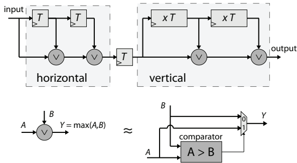
Fig. 3 3 \times 3 dilation unit for the geodesic pipeline.
