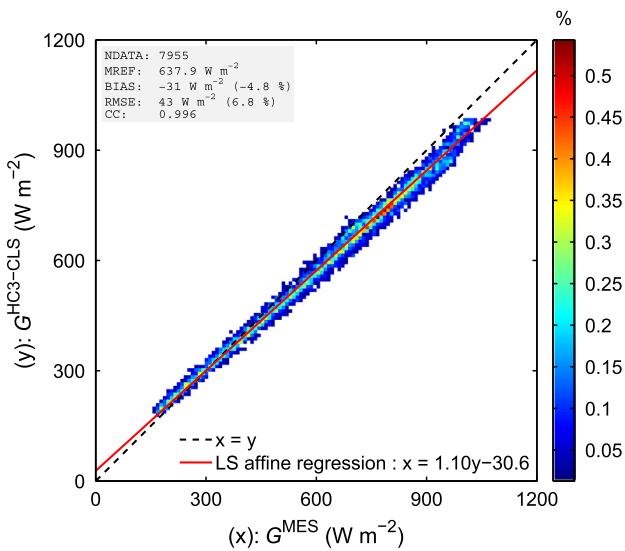
Fig. 12. Scatter density plot of HelioClim-3v4 ( G^{HC3-CLS} ) versus RSI ( G^{MES} ) global horizontal irradiance over Al Aradh, 2012.
