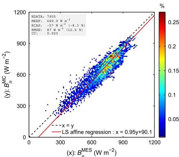
Fig. 3. Scatter density plot of McClear ( B_n^{MC} ) versus RSI ( B_n^{MES} ) direct normal irradiance over Al Aradh, 2012.
