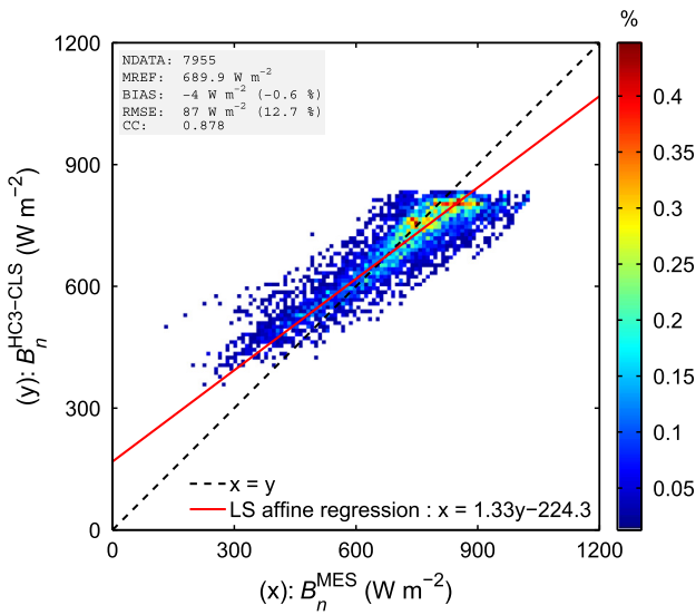
Fig. 16. Scatter density plot of HelioClim-3v4 ( B_n^{HC3-CLS} ) versus RSI ( B_n^{MES} ) direct normal irradiance over Al Aradh, 2012.
