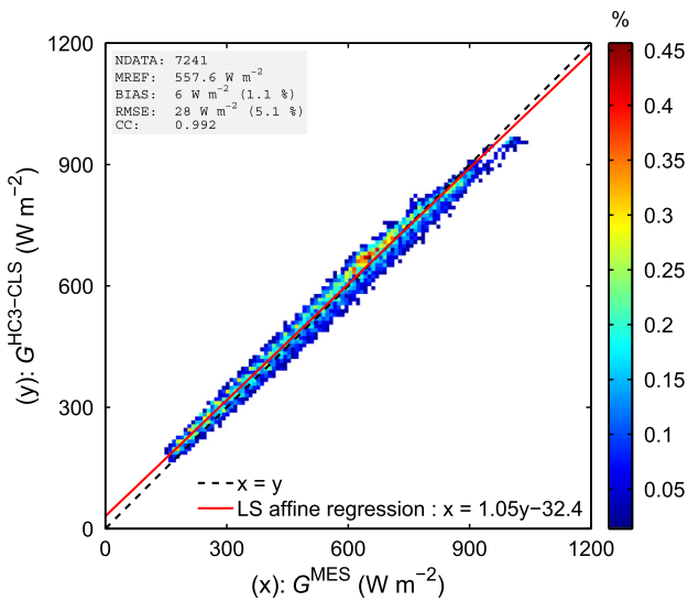
Fig. 13. Scatter density plot of HelioClim-3v4 ( G^{HC3-CLS} ) versus RSI ( G^{MES} ) global horizontal irradiance over Masdar City, 2012.
