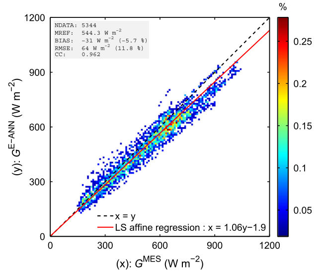
Fig. 15. Scatter density plot of E-ANN ( G^{E-ANN} ) versus RSI ( G^{MES} ) global horizontal irradiance over Masdar City, 2012.
