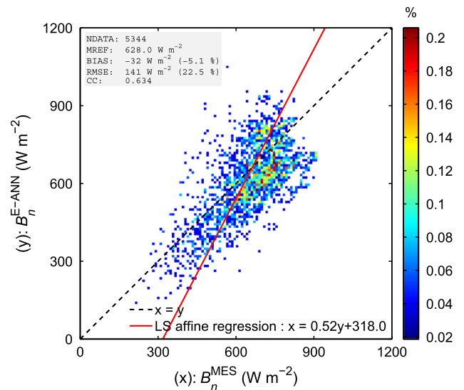
Fig. 19. Scatter density plot of E-ANN ( B_n^{E-ANN} ) versus RSI ( B_n^{MES} ) direct normal irradiance over Masdar City, 2012.
