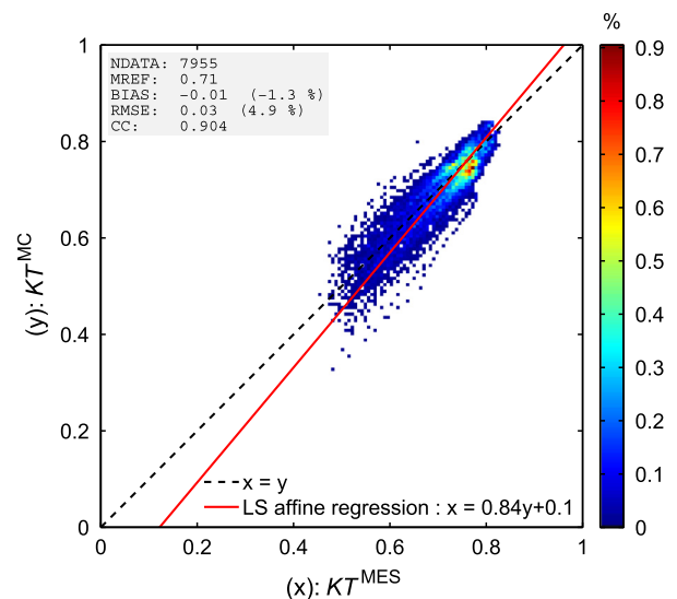
Fig. 4. Scatter density plot of McClear ( KT^{MC} ) versus RSI ( KT^{MES} ) clearness index over Al Aradh, 2012.
