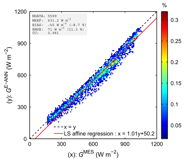
Fig. 14. Scatter density plot of E-ANN ( G^{E-ANN} ) versus RSI ( G^{MES} ) global horizontal irradiance over Al Aradh, 2012.
