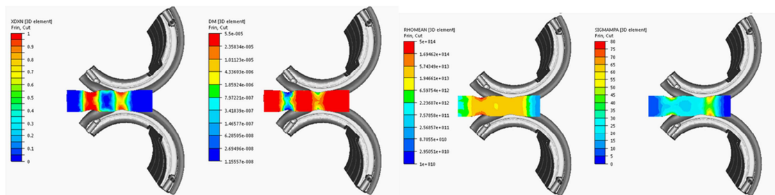
Fig. 11: Reducer-rolling simulation coupled with the mean-field model for microstructure evolution
