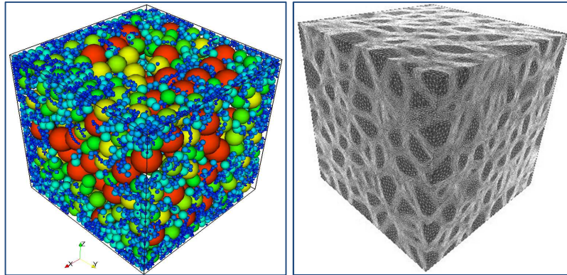
Fig. 14: REV respecting initial statistical data. Left a 304L powder. Right: 304L polycrystal with anisotropic finite element mesh in white.
