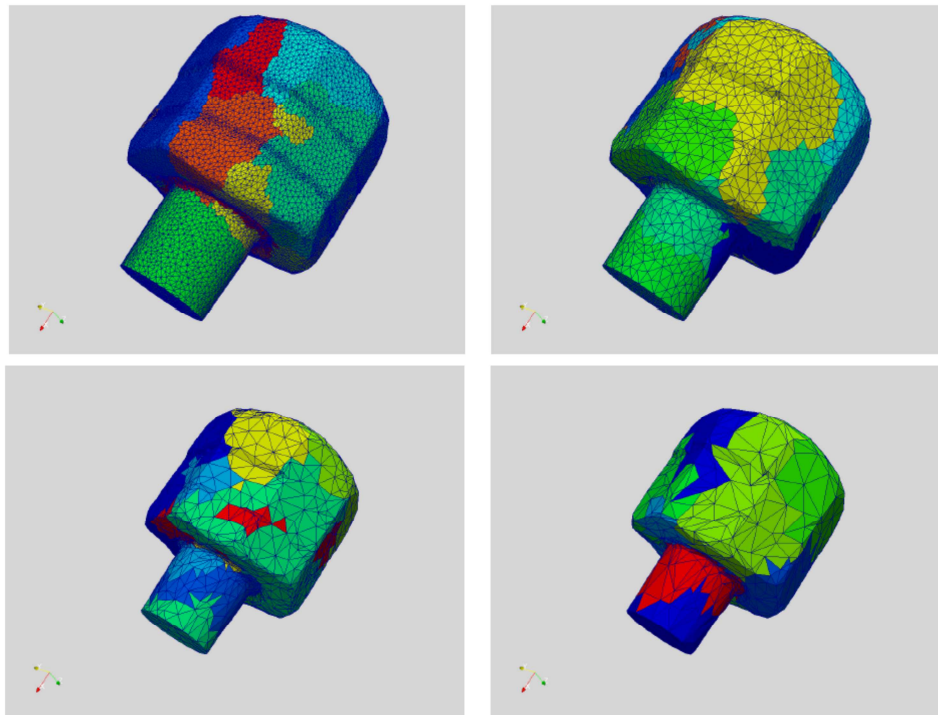
Fig. 10: Finer mesh (87 000 nodes) partitioned onto 12 processors for forging simulation (top left), and the intermediate meshes of 11 900 nodes, 3 800 nodes and 1 670 nodes for a four levels multigrid method.
