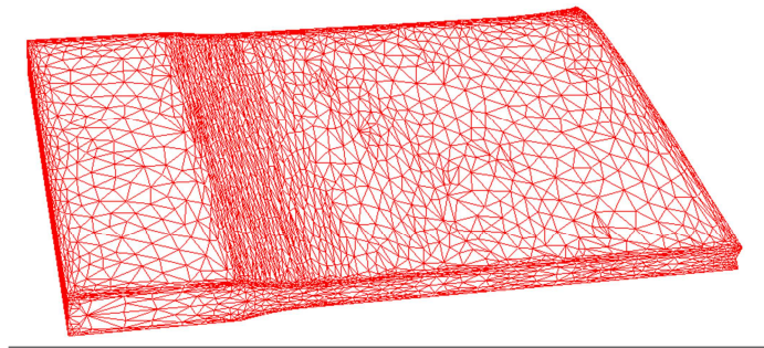
Fig. 2: anisotropic mesh for rolling
