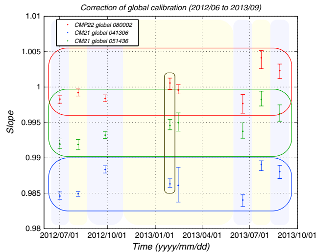
Figure 8. Corrections obtained by linear regression fit comparing pyranometer-derived DrHI (GHI – DfHI) with pyrhelimeter-derived DrHI. Corrections computed for the three pyranometers used in global mode are shown. Data within the blue and green rectangles are the corrections for the two CM21, and the data within the red rectangle are for the CMP22. For testing the changes over time of the calibration correction, data are aggregated in seven time periods including similar number of events (between 6000 and 12000 selected events). The time periods are shown as colored background. The fit for the whole period is also given in the middle of the study period surrounded by a vertical brown rectangle.
