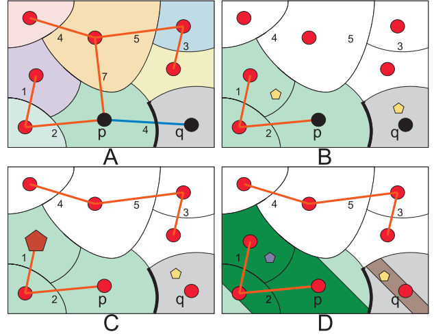
Fig. 7. A: Partition and its minimum spanning tree B: Area stochastic watershed: a random marker in both colored regions B_p and B_q C: Area oriented absorption stochastic watershed: a fixed marker in the largest region B_p and a random marker in the smaller region B_q D: Area stochastic watershed with transformed domains: a random marker in the regions obtained by a linear opening of B_p and B_q .
