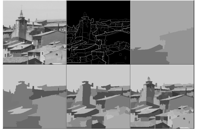
Fig. 8. The waterfall hierarchy. The saliency of the contours followed by 4 levels of the waterfall hierarchy.
