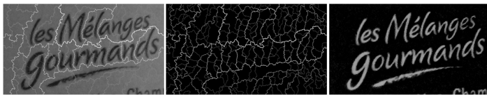
Fig. 9. Waterfall hierarchy used for the segmentation of text.
