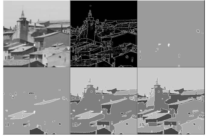
Fig. 3. An image, its watershed partition, followed by 4 levels of the ultrametric gradient hierarchy, going from coarse to fine.
