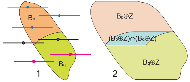
Fig. 6. 1: The two balls B_p and B_q and a number of structuring elements hitting the balls. The black ones hit both balls. 2: The dilated balls B_q \oplus Z and B_p \oplus Z and their intersection (B_q \oplus Z) \cap (B_p \oplus Z) in cyan colour.
