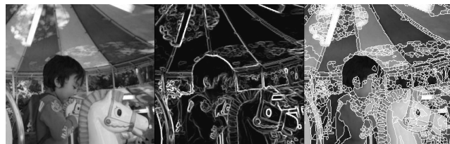
Fig. 1. A gray tone image, its gradient and the watershed segmentation associated to the minima of the gradient.
