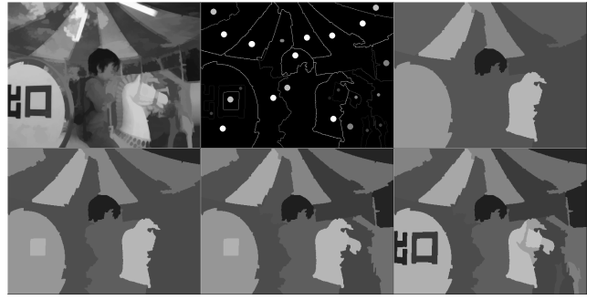
Fig. 4. A number of prioritized markers have been chosen: they appear as disks whose shade of grey is brighter for higher priorities. The associated hierarchy is illustrated through the saliency of the contours in the second image and through 4 levels of the associated hierarchy.
