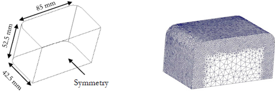
Figure 2: Slice geometry and finite element mesh.
