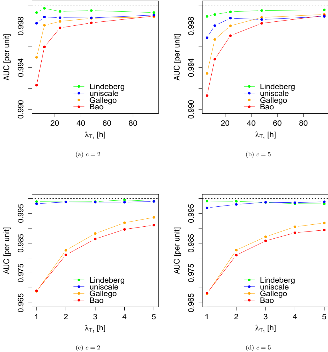
Figure 7: Optimal detection performance depending on average inter-ramps' duration – Maximum AUC (i.e., for a maximum scale parameter value s_n^* = \operatorname{argmax}_{s_n} \operatorname{AUC}(\lambda_{T_1}, c) ), depending on the average duration of an episode of low production \lambda_{T_1} and the ratio defining the average duration of an episode of high production c , for multi-scale approaches: Gallego, Bao and Lindeberg. Graphs on top are for parameter values \lambda_{T_1} = 6, 12, 24, 48, 96 h, while graphs at the bottom correspond to values \lambda_{T_1} = 1, 2, 3, 4, 5 h. Performance when using a single globally optimal scale for detecting all the ramps in a signal (blue curve), is here given as a reference. It allows for a clear discrimination between an approach's performance based on a local scale selection procedure (i.e., Lindeberg), and those based on scales' combination (i.e., Bao and Gallego).
