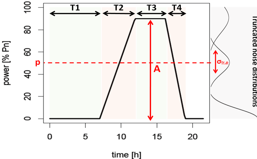
Figure 1: Elementary ramp profile and noise distribution – Diagram showing an elementary ramp profile R^k defined by Equation (3). Represented here are: the amplitude A of a ramp, the duration T_i , i = 1, \dots, 4 of ramps and periods between consecutive ramps, and the distribution of the noise associated to a production level p in R^k . Power level is expressed in percentage of the nominal power P_n .
