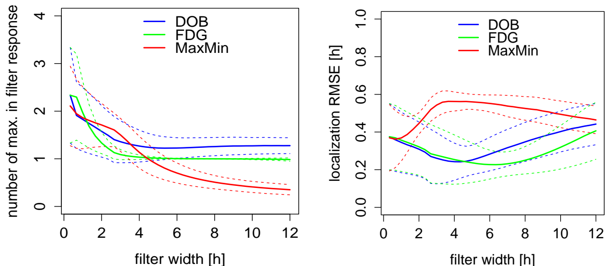
Figure 6: Filter’s responses multiplicity and ramps localization error – Multiplicity of maximum in the response of a filter to a ramp (graphic on the left), and root mean square of the ramp localization error (graphic on the right), for the DOB, FDG and MaxMin filters, depending on the filter’s width. Increasing the filter’s width reduces the multiplicity of responses to a ramp. In the case of the MaxMin filter, this is not due to noise reduction, as it is for the DOB and FDG filters, but to its propensity for maintaining its maximum value. The MaxMin filter’s noise sensitivity causes a rapid increase of a ramp’s localization error with the filter’s width. If this error decreases for filter’s higher widths, this is due to the fact that errors higher than \delta , have not been taken into account when computing the average localization error.
