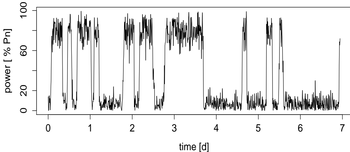
Figure 4: Simulation example – production episode lasting 7 days simulated from the proposed ramp model. Here, the amplitude of ramps is set at A = 80\%P_n . Ramps are, on average, of short duration, i.e., \lambda_{T_2} = 1/2 h, and rather close to one another \lambda_{T_1} = 12 h. The characteristic ratio between the duration of low and high production episodes has been set at c = 2 , while noise of high intensity has been added to the ramp profile (see text for more details).
