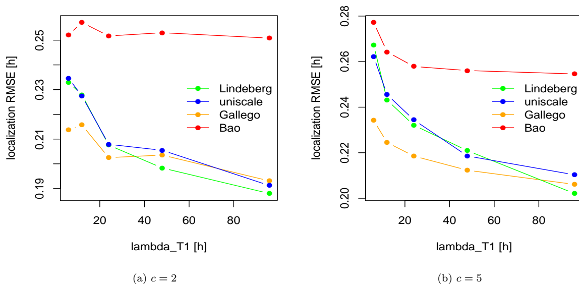
Figure 9: Optimal localization performances depending on average inter-ramps' duration – Ramp localization root mean squared error of the considered detection approaches, depending on the inter-ramps' duration parameters \lambda_{T_1} and c . These results contrast those obtained for detection, since it is the Gallego scales' combination approach which performs the best for close consecutive ramps.
