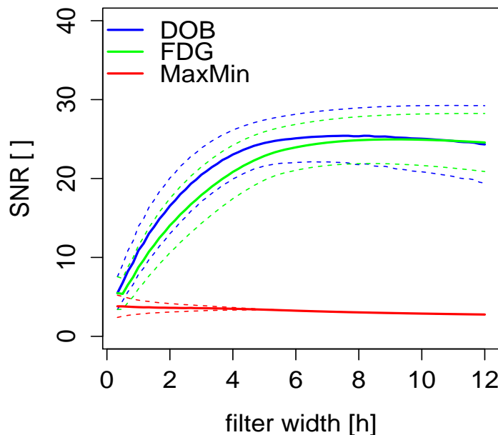
Figure 5: Signal-to-noise ratio at filter’s output (Canny’s first criterion) – Average ratio (solid lines), + / - standard deviation (dashed lines) for DOB, MaxMin and FDG filters, depending on the filter’s width. Filter’s width here ranges from 20 min to 12 h. Noise attenuation from the smoothing operation performed by the DOB and FDG filters allows for a rapid increase in detection performance when the filter’s width increases. The presence of nearby ramps limits the response to a ramp, and ultimately results in SNR stagnation for a filter’s higher width value. Due to the particular nature of its definition, the MaxMin filter’s response to noise increases with the filter’s width. This increase counterbalances the one associated with the filter’s response to a ramp, thus resulting in an overall low level of SNR.
