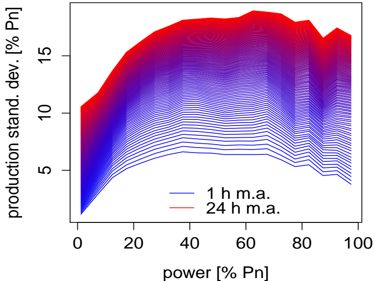
Figure 3: Production standard deviation as a function of the production level – Empirical estimates of the production standard deviation computed from sliding windows with width ranging from 1 h to 24 h, with 20 minutes’ increment. One can observe how the production distribution tends to spread out, while the production level increases. The production standard deviation tends to stagnate or even decrease here, when the production level comes closer to the wind farm’s nominal capacity.
