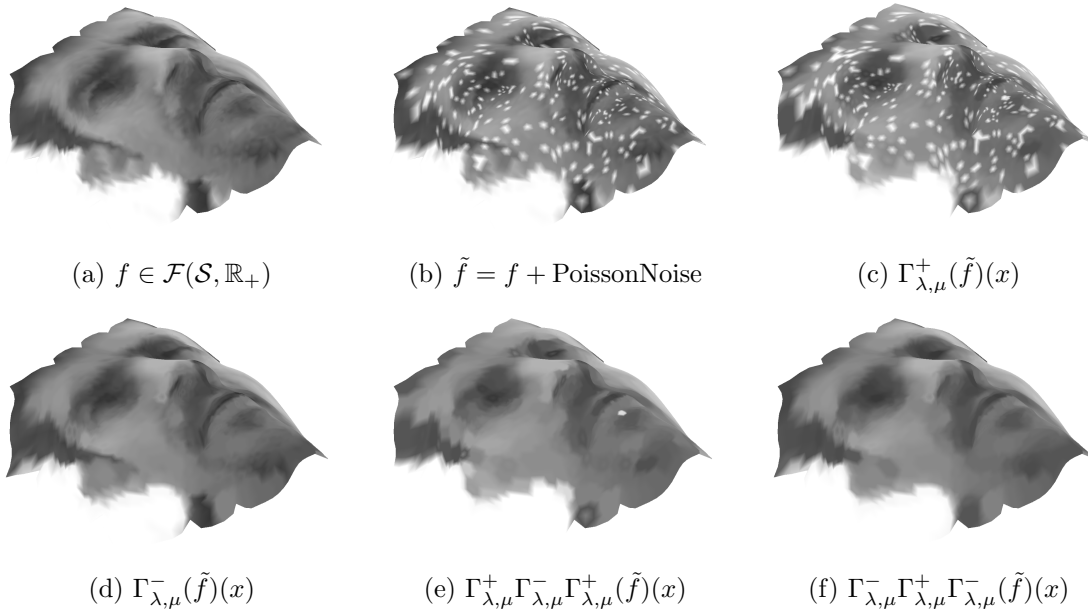
Figure 5: Restoring image missing parts: Original image (a) has been corrupted with Poisson noise in (b). From (c) to (f), filtered image by composition of different Lasry-Lions regularizers (for all the cases \lambda = 1/2 ; \mu = 1/4 ).
