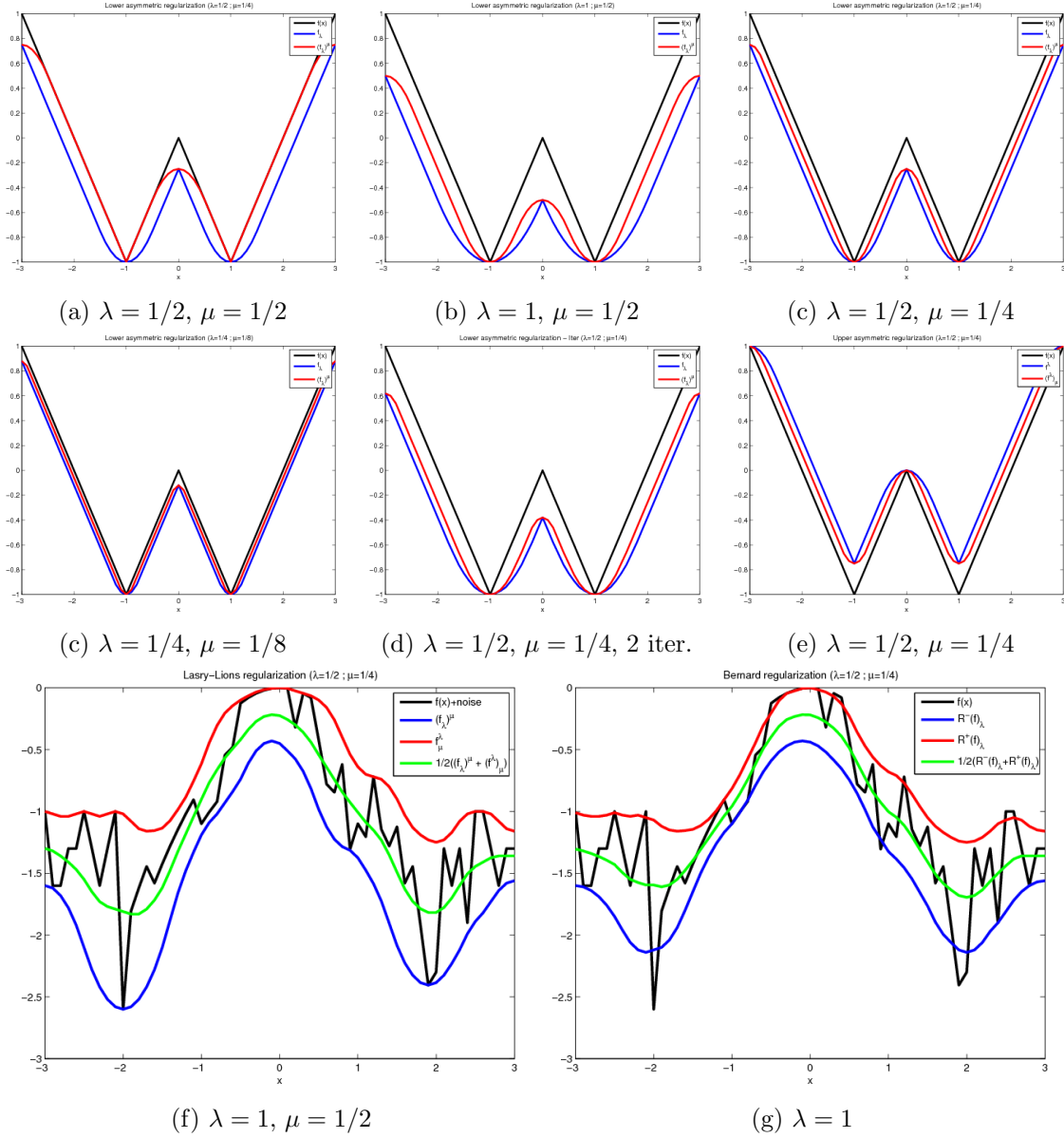
Figure 3: Lasry-Lions regularization of a 1D signal (original signal in black, operator in \lambda in blue and composed operator in \mu in red: (a) quadratic opening, (b) to (c) lower regularizer (f_\lambda)^\mu , (d) iterated lower regularizer, (e) upper regularizer (f^\lambda)_\mu . Bottom row, comparison between Lasry-Lions regularizers (f) and Bernard regularizers (g). Green curves correspond to the averages.
