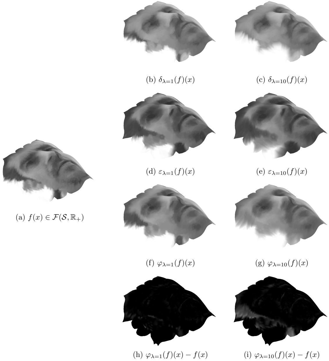
Figure 2: Morphological operators applied on a real-valued function on a smooth surface: (a) original image f : S \rightarrow \mathbb{R} , (b) and (c) canonic Riemannian dilation \delta_\lambda(f) with \lambda = 1 and \lambda = 10 , (d) and (e) canonic Riemannian erosion \varepsilon_\lambda(f) with \lambda = 1 and \lambda = 10 , (f) and (g) canonic Riemannian closing \varphi_\lambda(f) with \lambda = 1 and \lambda = 10 , (h) and (i) residues between the original image f and the closings \varphi_\lambda(f) .
