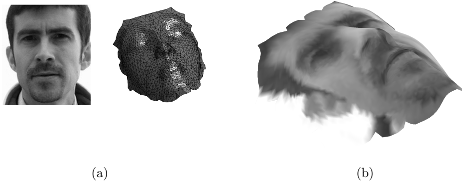
Figure 1: (a) Euclidean real-valued function + smooth surface (as a discrete mesh); (b) real-valued function on smooth surface.
