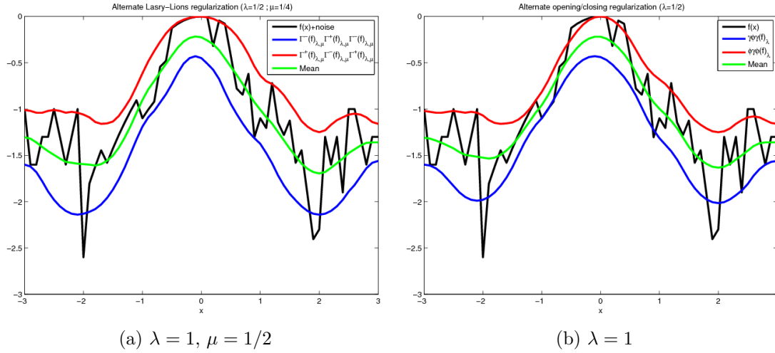
Figure 4: Comparison between alternate Lasry–Lions regularizers (a) and classical alternate morphological filters (b).
