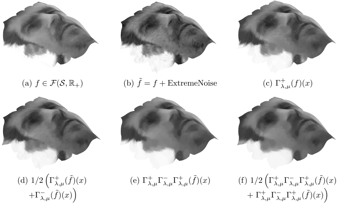
Figure 6: Restoring image acquisition noise: Original image (a) has been corrupted with non-Gaussian noise in (b). From (c) to (f), filtered image by composition of different Lasry-Lions regularizers (for all the cases \lambda = 1/2 ; \mu = 1/4 ).
