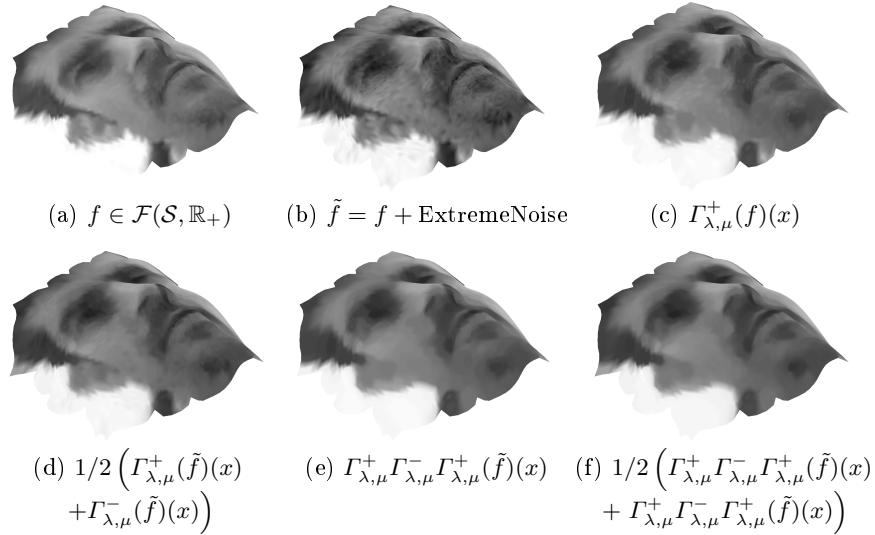
Fig. 6. Restoring image acquisition noise: Original image (a) has been corrupted with non-Gaussian noise in (b). From (c) to (f), filtered image by composition of different Lasry-Lions regularizers (for all the cases \lambda = 1/2 ; \mu = 1/4 ).
