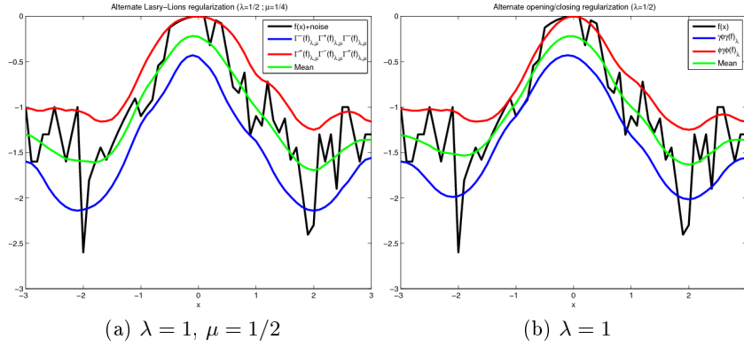
Fig. 4. Comparison between alternate Lasry-Lions regularizers (a) and classical alternate morphological filters (b).
