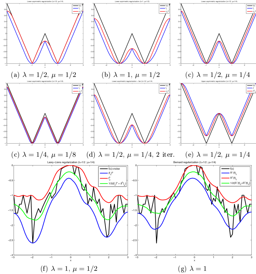
Fig. 3. Lasry-Lions regularization of a 1D signal (original signal in black, operator in \lambda in blue and composed operator in \mu in red: (a) quadratic opening, (b) to (c) lower regularizer (f_\lambda)^\mu , (d) iterated lower regularizer, (e) upper regularizer (f^\lambda)_\mu . Bottom row, comparison between Lasry-Lions regularizers (f) and Bernard regularizers (g). Green curves correspond to the averages.
