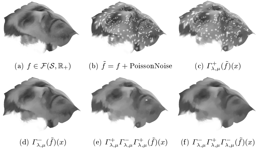
Fig. 5. Restoring image missing parts: Original image (a) has been corrupted with Poisson noise in (b). From (c) to (f), filtered image by composition of different Lasry-Lions regularizers (for all the cases \lambda = 1/2 ; \mu = 1/4 ).
