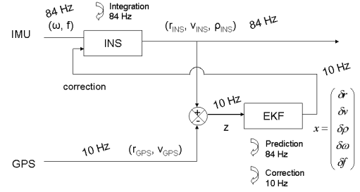
Figure 5: GPS-INS coupling
