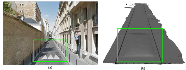
Fig. 4. Surface reconstruction results obtained for the dataset Cassette. (a) Google street view of the surveyed area; (b) N_p = 1.01 Mpts, N_t = 2.026 MTriangles, decimated mesh with f_D = 90\% , NDT = 203k Triangles.
