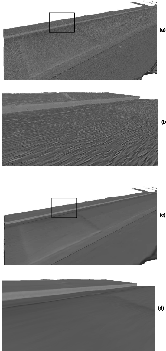
Fig. 3. Mesh smoothing results on dataset Cassette acquired over Cassette street situated in Paris, (France) by the STEREOPLIS MMS [Pap14] equipped with a Riegl sensing device. (a) planar Delaunay triangulation, (b) zoom-in view on the sidewalk border corresponding to the black rectangle area illustrated in Fig. (a); (c) the result of the Sinc windowed smoothing procedure; (d) zoom-in view on the sidewalk border corresponding to the black rectangle area illustrated in Fig. (c).
