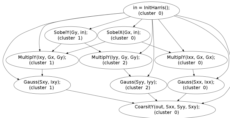
Figure 12: Hierarchically scheduled SDG for Harris, using P=3 cores
