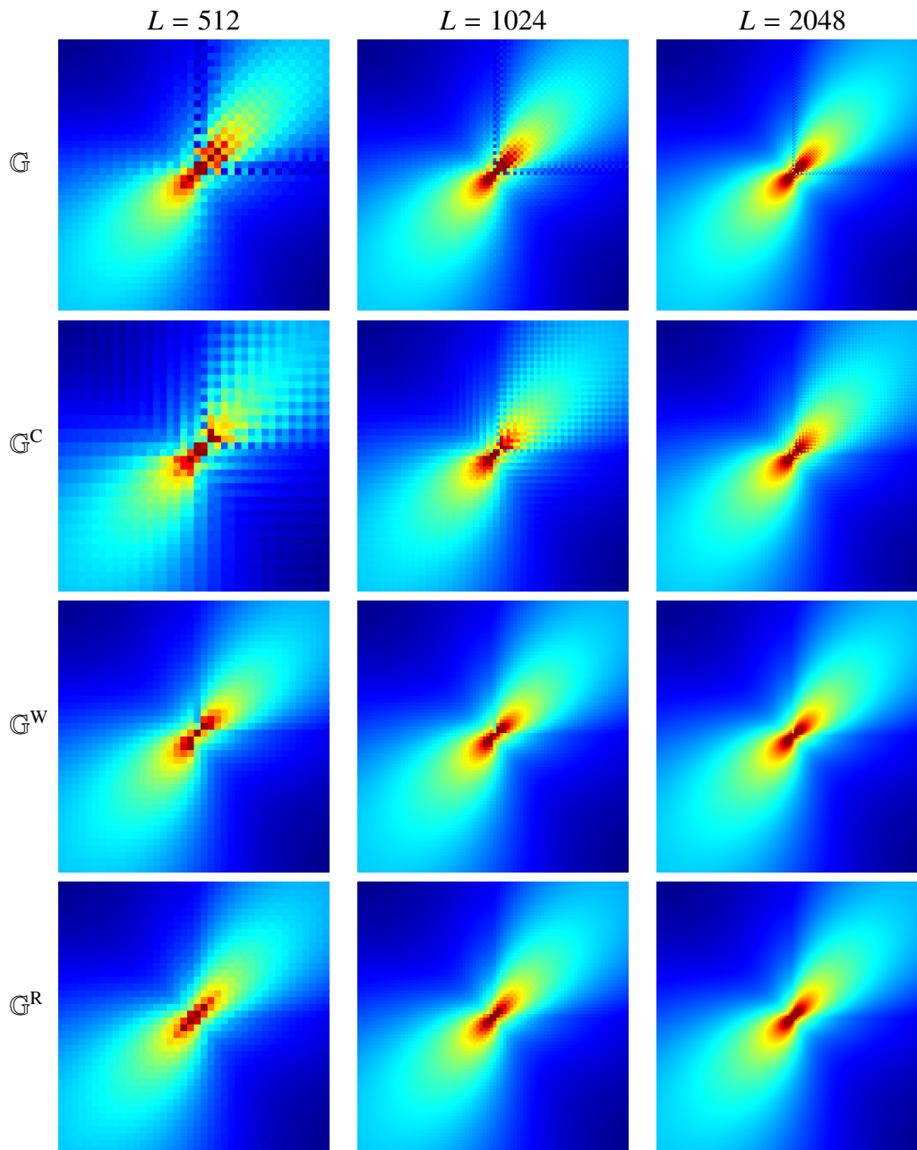
Figure 3: Stress component \sigma_{12}(\mathbf{x}) predicted by the various FFT schemes at the three resolutions L = 512, 1024 and 2048 (left to right) in the region [-0.04; 0.04]^2 . The center of the region is the bottom-left corner of the square inclusion in Fig. (2).
