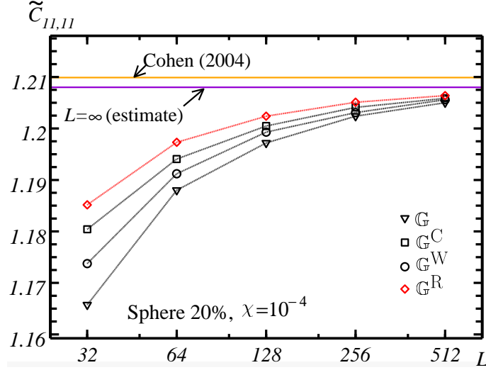
Figure 5: Apparent elastic modulus \tilde{C}_{11,11} estimated by FFT methods using the Green operators \mathbb{G} and \mathbb{G}^{C,W,R} (black and red), at increasing resolution L . Orange: estimate in [28]; violet: estimate of the asymptotic effective modulus \tilde{C}_{11,11} using FFT data.
