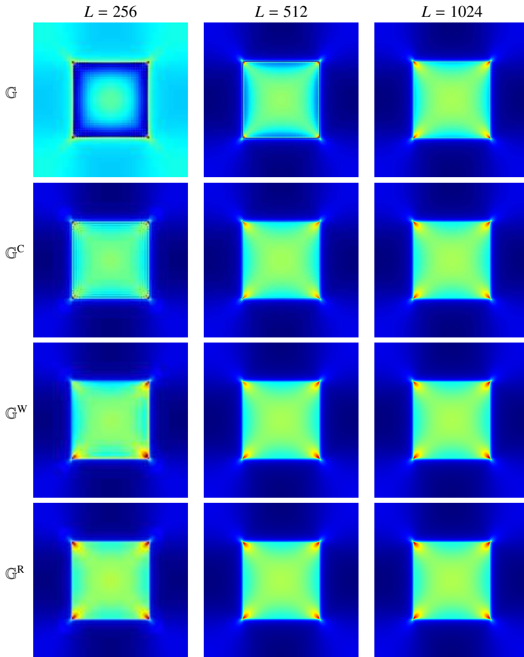
Figure 4: 2D section of the stress component \sigma_{12}(\mathbf{x}) along the plane x_3 = -0.2461 predicted by the various FFT schemes at the three resolutions L = 256 , L = 512 and L = 1024 (left to right). The section is parallel to one of the faces of the inclusion and close to the interface with the matrix.
