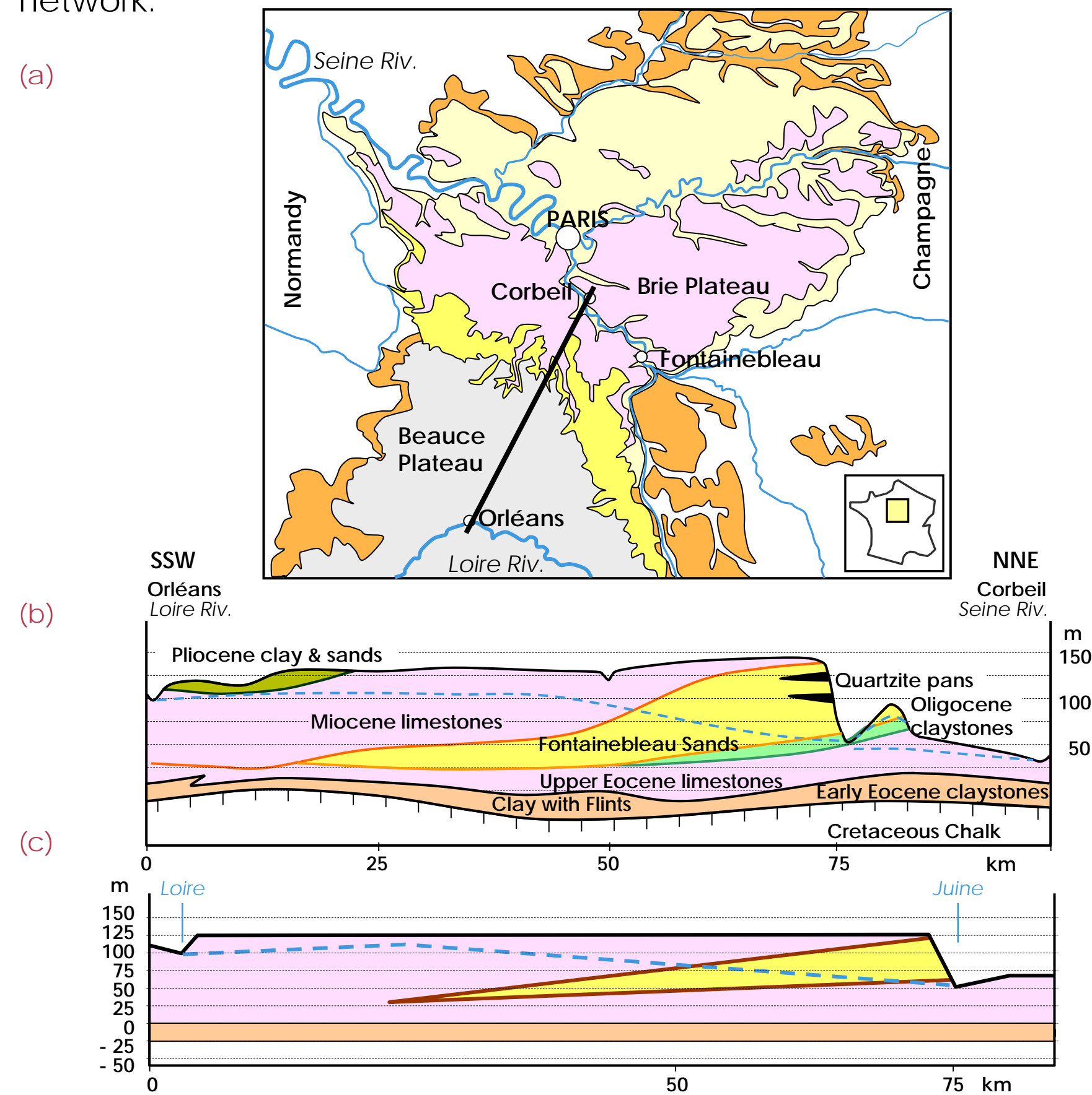
Fig. 1 - Hydrogeologic framework
