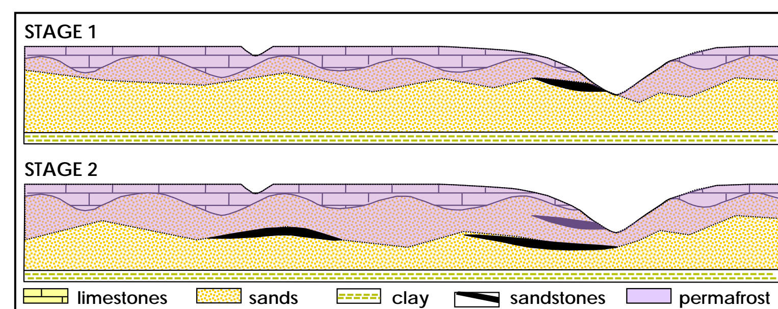
Fig. 7 - Model of silicification associated with a cold front propagation During cold periods of the Quaternary, silicification would occur at the abrupt temperature interface between permafrost and warmer groundwater.
