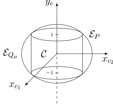
Fig. 3. Inclusion of \mathcal{E}_P within \mathcal{E}_{Q_\mu}
