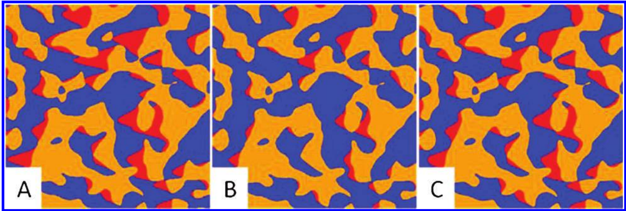
7 Shadow PGS: Influence of the parameters. Reference outcome (A); Increased incidence angle (B); Decreased maximum threshold (C)
