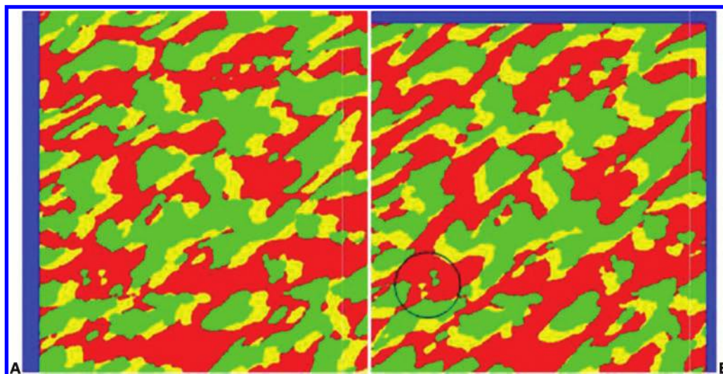
4 Shifted PGS. The model for the first GRF is an anisotropic cubic structure. The second GRF is a shift of the first one. The shift is equal to [15 m, 0] (A) and [-10 m, -10 m] (B)
