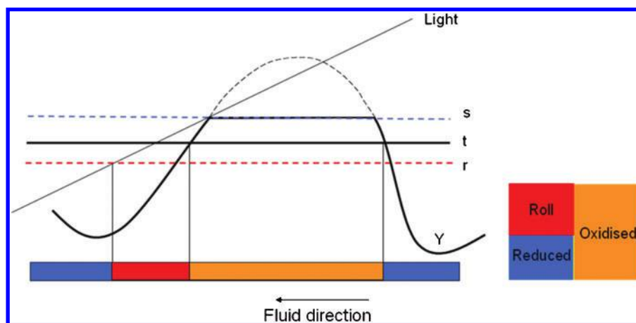
5 Explanation scheme for the Shadow PGS
