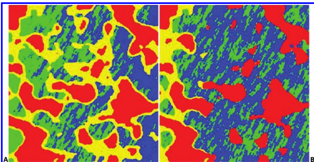
3 Non-stationary PGS: (A) Red and Yellow constant (25%): Blue increases and Green decreases from left to right, (B) Red and Green constant (25%): Blue increases and Yellow decreases from left to right
