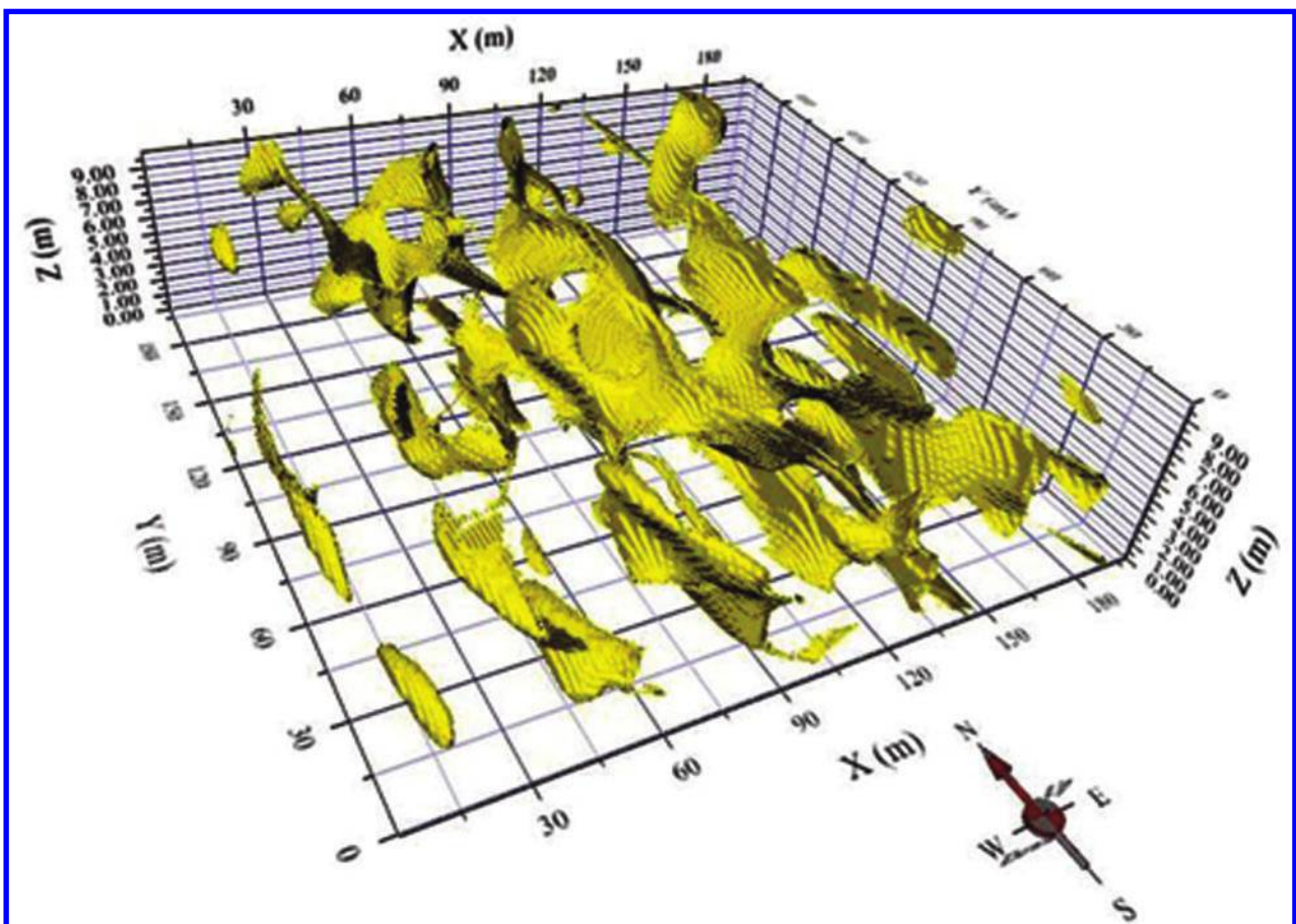
8 Roll front simulated using shadow PGS
