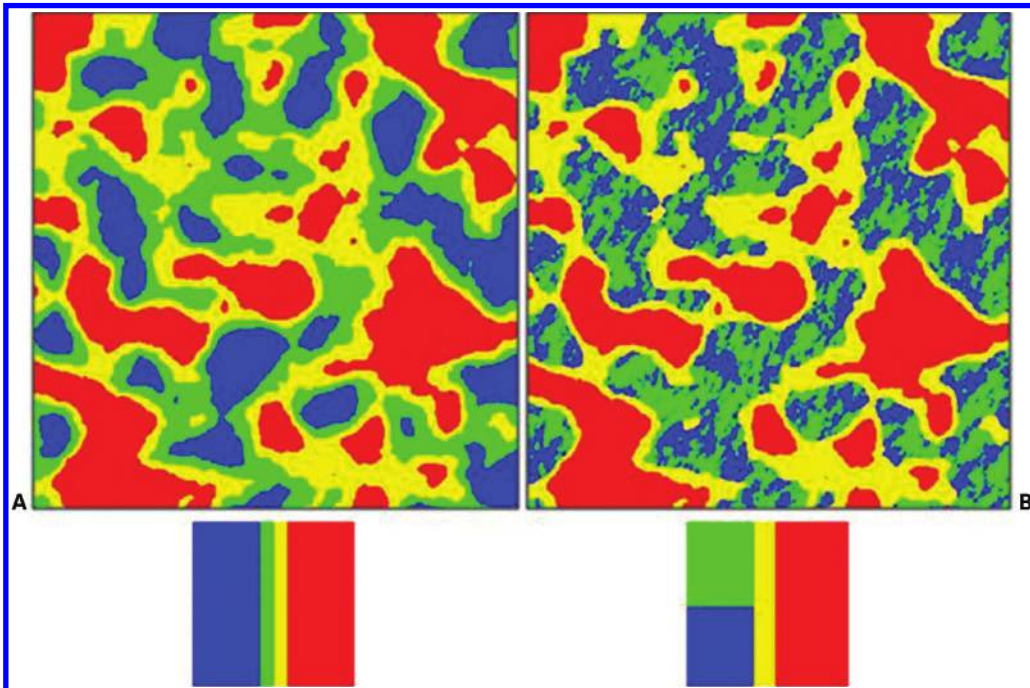
2 Outcomes with four facies (same proportion=25%): MonoGaussian (A) and PluriGaussian (B) – Lithotype rules (second line): contact between blue–green and red facies is forbidden. First GRF: cubic variogram; Second GRF: exponential anisotropic (N30) variogram
