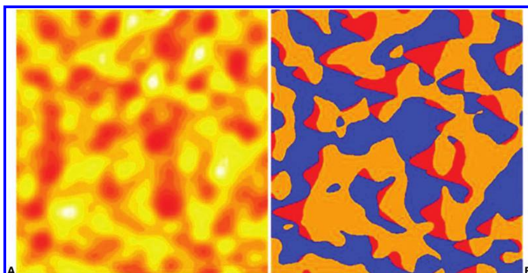
6 Shadow PGS: Gaussian simulation outcome (A) and Shadow PGS (B)
