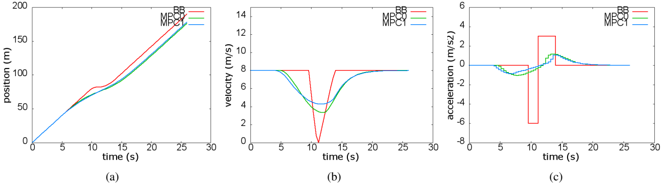
Fig. 6: Vehicle 3: position (left), velocity (middle) and acceleration (right) profiles under three different control strategies. MPC 1 leads to less velocity drop than MPC 0 thanks to more precise prediction of prior vehicles' future states.
