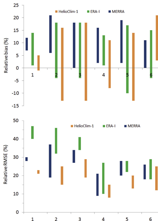
Fig. 6. Ranges of relative bias (top) and relative RMSE (bottom) for each climatic area and each database. Daily clearness index. Area 1) Baltic Area, 2) France, 3) Eastern Europe, 4) North Africa, 5) Mozambique, and 6) Equatorial Atlantic Ocean.
