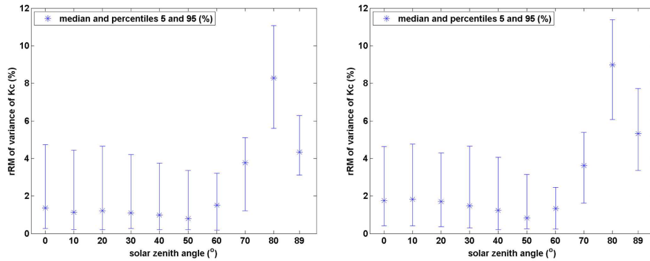
Figure 4. Median (star) and 5th and 95th percentiles of \text{RM}(v(K_c)) relative to the corresponding mean K_c for all couples (\rho_g, \tau_c) as a function of \theta_S for water cloud (left) and ice cloud (right).
