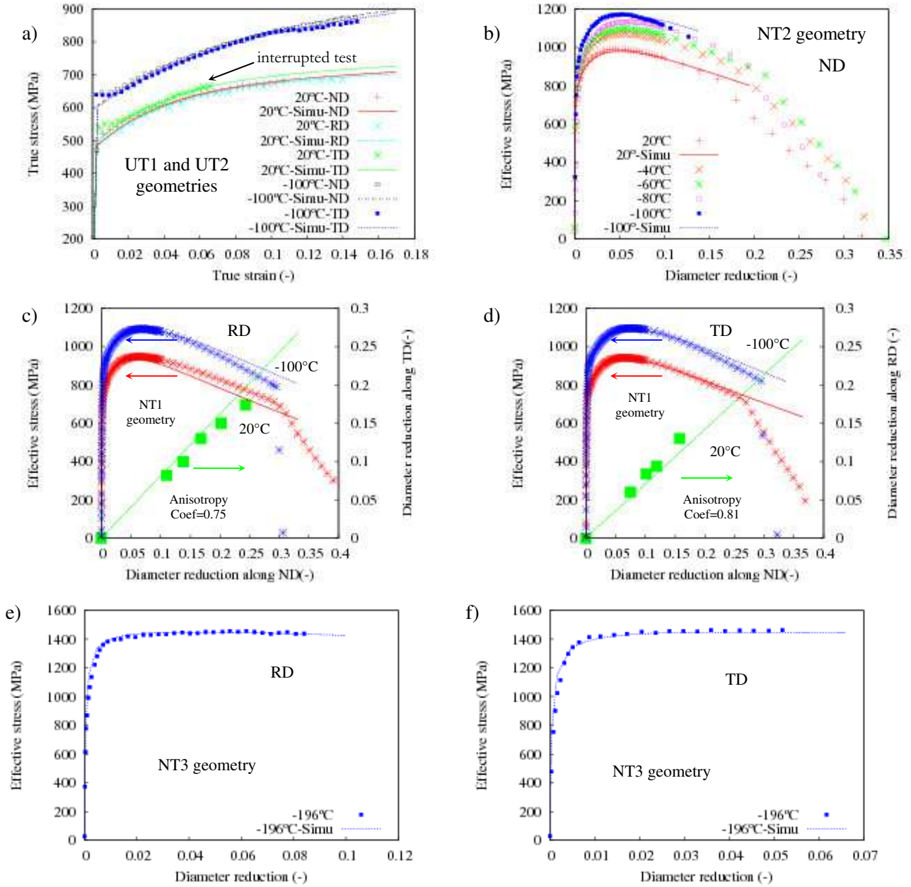
Fig. 2. Tensile curves of (a) smooth, (b)–(f) notched specimens. Symbols: experiments; lines: model predictions.
