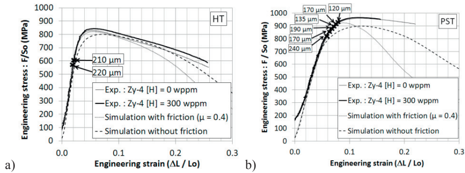
Fig. 3. Engineering stress-strain curves for non-hydrided and hydrided (a) HT tests (b) PST tests, containing blisters or not. Crosses indicate the failure of samples containing a blister, blister depths are given in the boxes.
