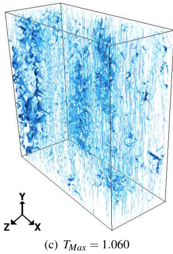
Fig. 25. Reconstruction of the paths by backtracking in 26-connectivity after thresholding the morphological tortuosity in the Oy direction for the pores of Thermisorel™.
