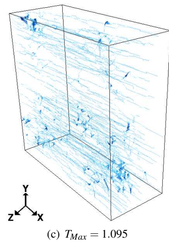
Fig. 24. Reconstruction of the paths by backtracking in 26-connectivity after thresholding the morphological tortuosity in the Ox direction for the pores of Thermisorel TM .
