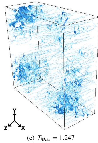
Fig. 26. Reconstruction of the paths by backtracking in 26-connectivity after thresholding the morphological tortuosity in the Oz direction for the pores of Thermisorel™.
