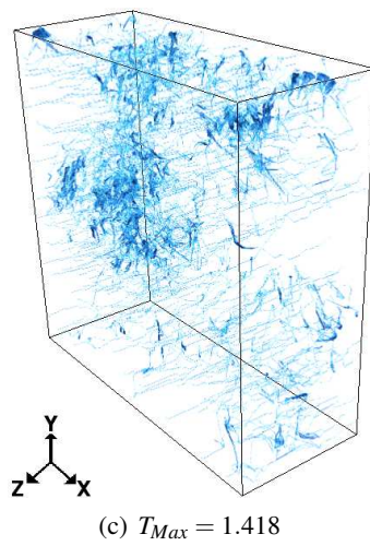
Fig. 23. Reconstruction of the paths by backtracking in 26-connectivity after thresholding the morphological tortuosity in the Oz direction for the fibres of Thermisorel TM .
