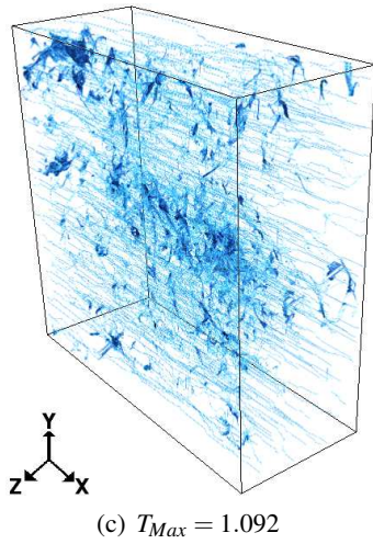
Fig. 21. Reconstruction of the paths by backtracking in 26-connectivity after thresholding the morphological tortuosity in the Ox direction for the fibres of Thermisorel™.
