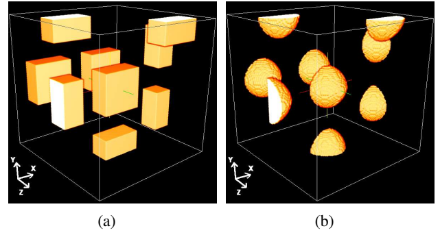
Fig. 5. 3D structuring elements of size 15 propagating in the Oz+ direction on the point-pattern of Fig. 4. (a) Half cubes, (b) Half spheres.
