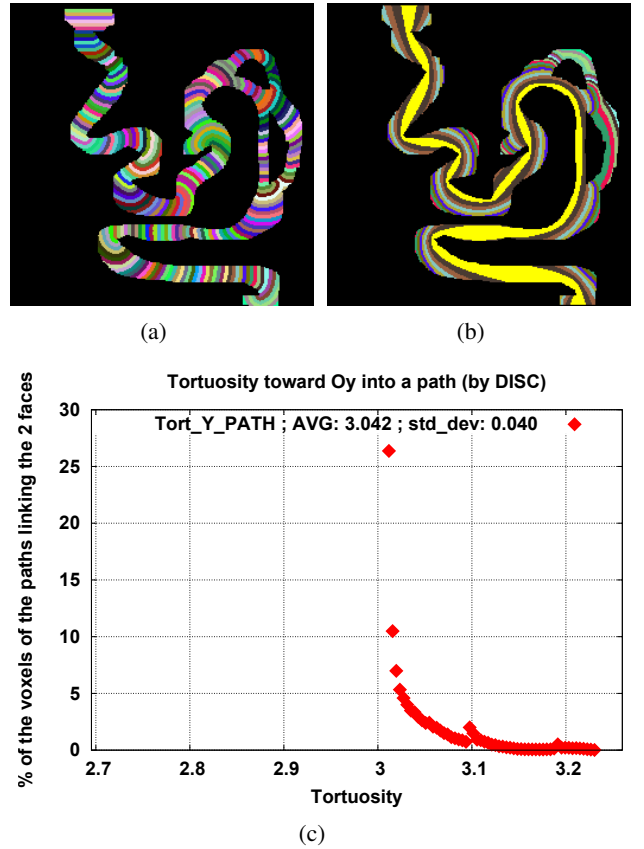
Fig. 8. Estimation, from propagations of discs, of the tortuosities of the 2D white part of Fig. 3. (a) Forward propagation, (b) Image of the tortuosities (minimum tortuosity: 3.01 in yellow), (c) Histogram of the tortuosities.
