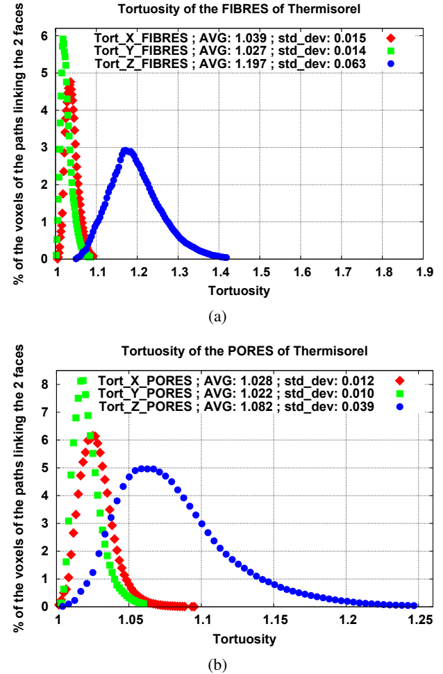
Fig. 20. Histograms of the morphological tortuosities (a) into the fibres and (b) into the pores of Thermisorel™ in Fig. 19 in the Ox, Oy and Oz directions.
