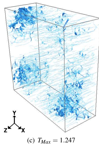
Fig. 26. Reconstruction of the paths by backtracking in 26-connectivity after thresholding the morphological tortuosity in the Oz direction for the pores of Thermisore\Gamma^M .
