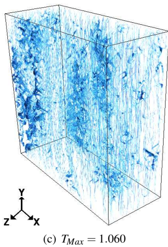
Fig. 25. Reconstruction of the paths by backtracking in 26-connectivity after thresholding the morphological tortuosity in the Oy direction for the pores of Thermisore\Gamma^M .
