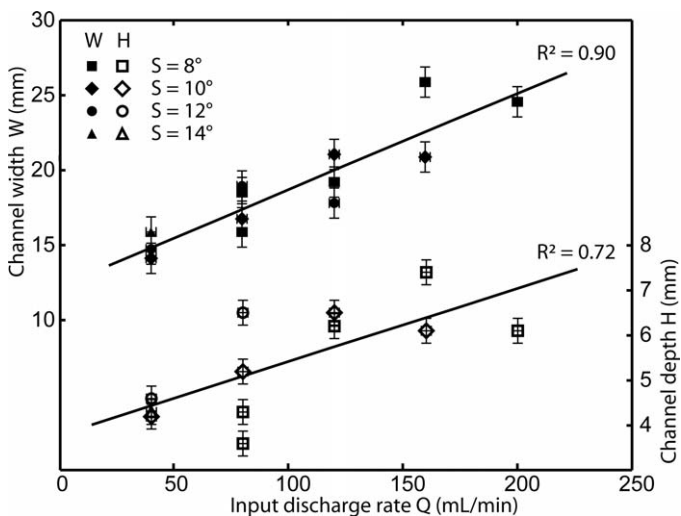
FIG. 11.—Steady-state channel width (full symbols) and depth (empty symbols) as a function of the discharge. The symbols represent the initial slope. Error bars are 4 \text{ mL} \cdot \text{min}^{-1} for the discharge rate, 2 \text{ mm} for the channel width, and 0.5 \text{ mm} for the channel depth.
