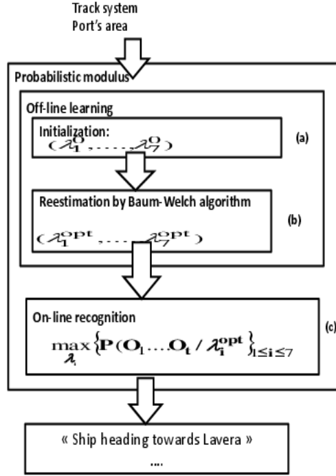
Figure 4: Probabilistic modulus
