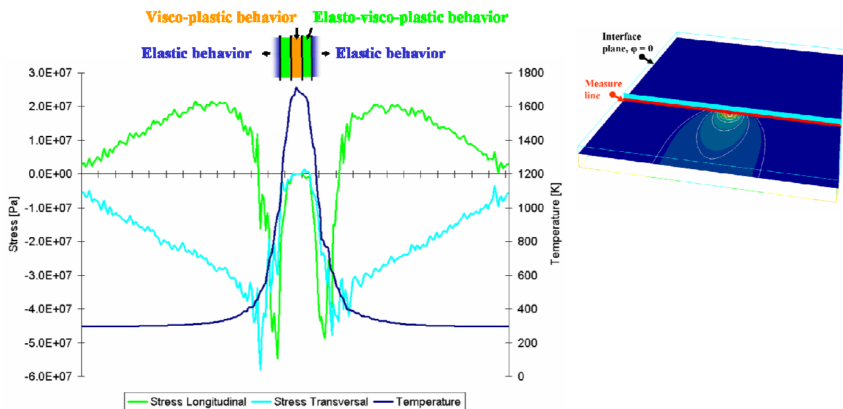
FIGURE 10: Evolution of the interface stresses according to the torch distance.
