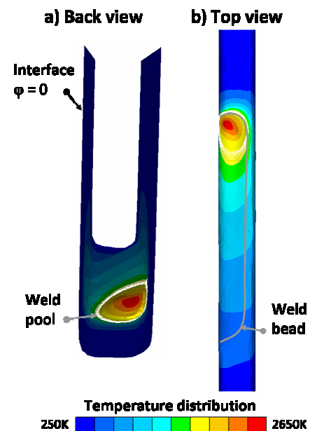
FIGURE 4: Two views of the numerical weld bead. Temperature distribution at the interface.
