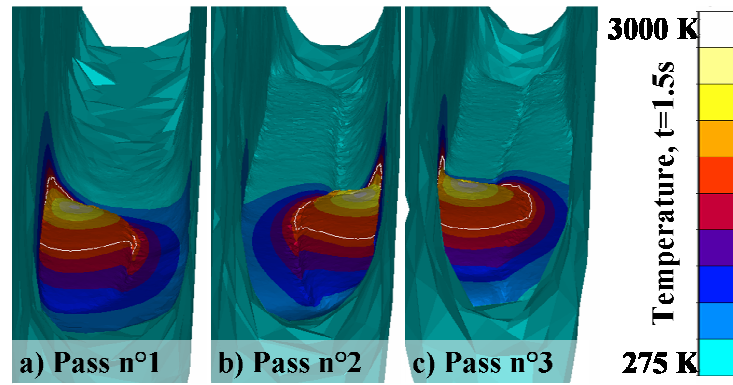
Fig. 8: The first a), second b) and third c) passes formed for the same time t = 1.5s after each pass has started. The temperature field is superimposed at the weld bead surface. The white line corresponds to the liquidus temperature.
