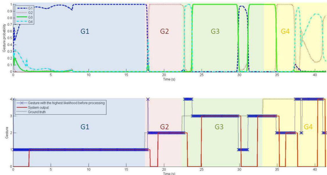
Figure 5: On top, gesture probabilities output in real-time by our recognition system. On bottom, the gesture with the highest probability in real-time (blue), the final result (estimate of performed gesture) obtained after time-window filtering (red), and the ground truth (black). The four performed gestures are successively G1, G2, G3 and G4. Their time intervals are represented with color background: blue for G1, red for G2, green for G3 and yellow for G4.
