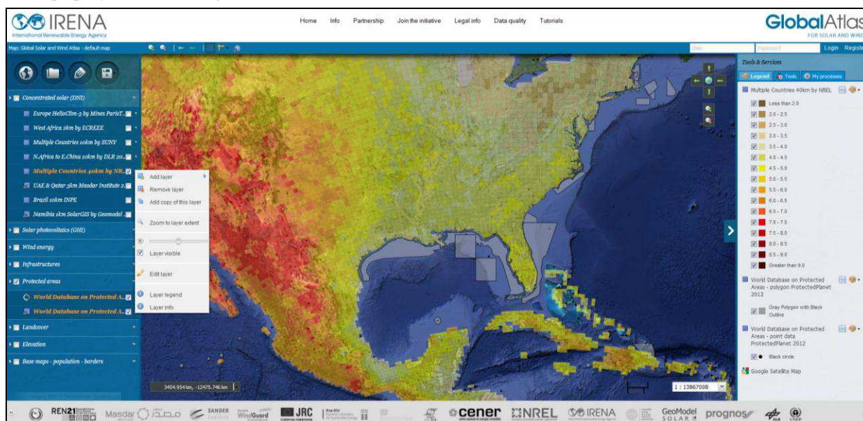
Figure 3 - GIS Interface
