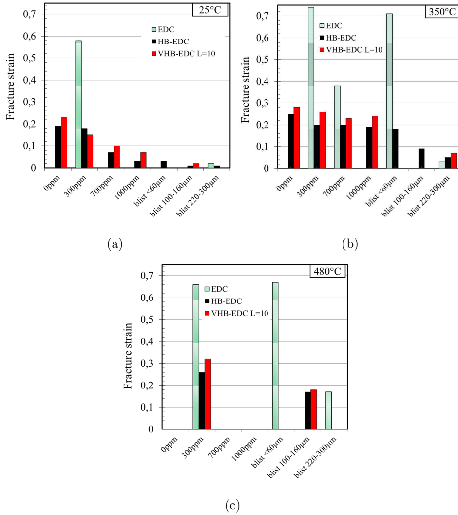
Figure 4: Fracture strain measured in EDC, HB-EDC and VHB-EDC L=10 at (a) 25 °C, (b) 350 °C and (c) 480 °C.
