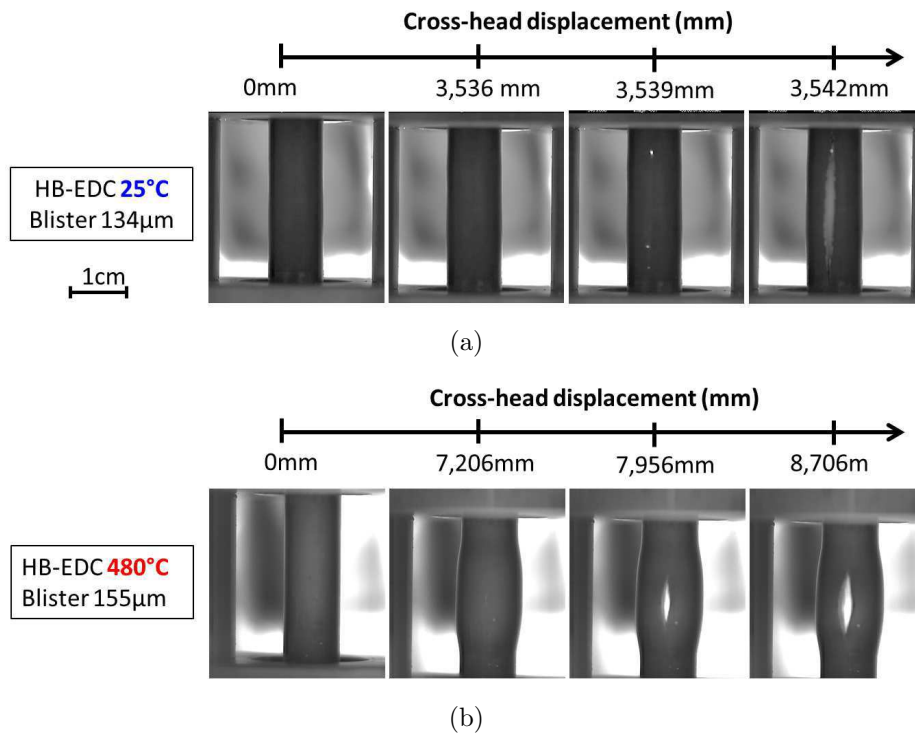
Figure 9: Video monitoring of an HB-EDC test with an about 150 \mu\text{m} deep blister at (a) 25 °C and (b) 480 °C.
