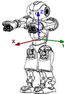
Figure 2: Axes definition on the robot
