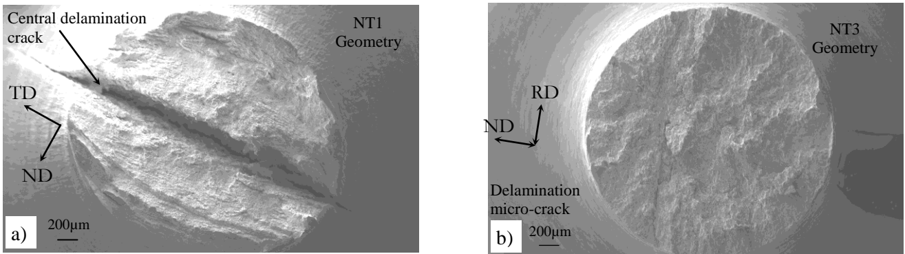
FIG. 3 – Fracture surfaces (a) of a NT1 specimen (RD, -100°C) and (b) of a NT3 specimen (TD, -196°C)
