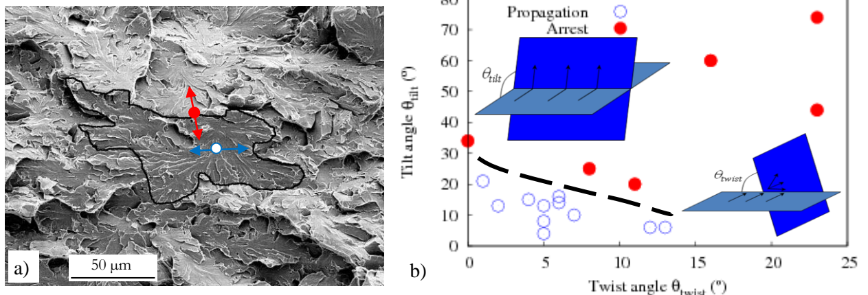
FIG. 5 – (a) Fracture surface of an NT2 specimen tested along ND at -100°C. (b) Local cleavage propagation or arrest according to measured tilt and twist components of misorientation (region delineated in black in (a))
