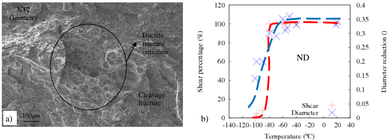
FIG. 4 – (a) Fracture surface of a NT2 specimen (ND, -90°C). (b) Evolution of the shear percentage and diameter reduction (at fracture) with testing temperature (NT2 specimens tested along ND).
