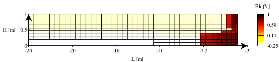
Scenario 2 – Eh (pyrite rate \times 10 )
