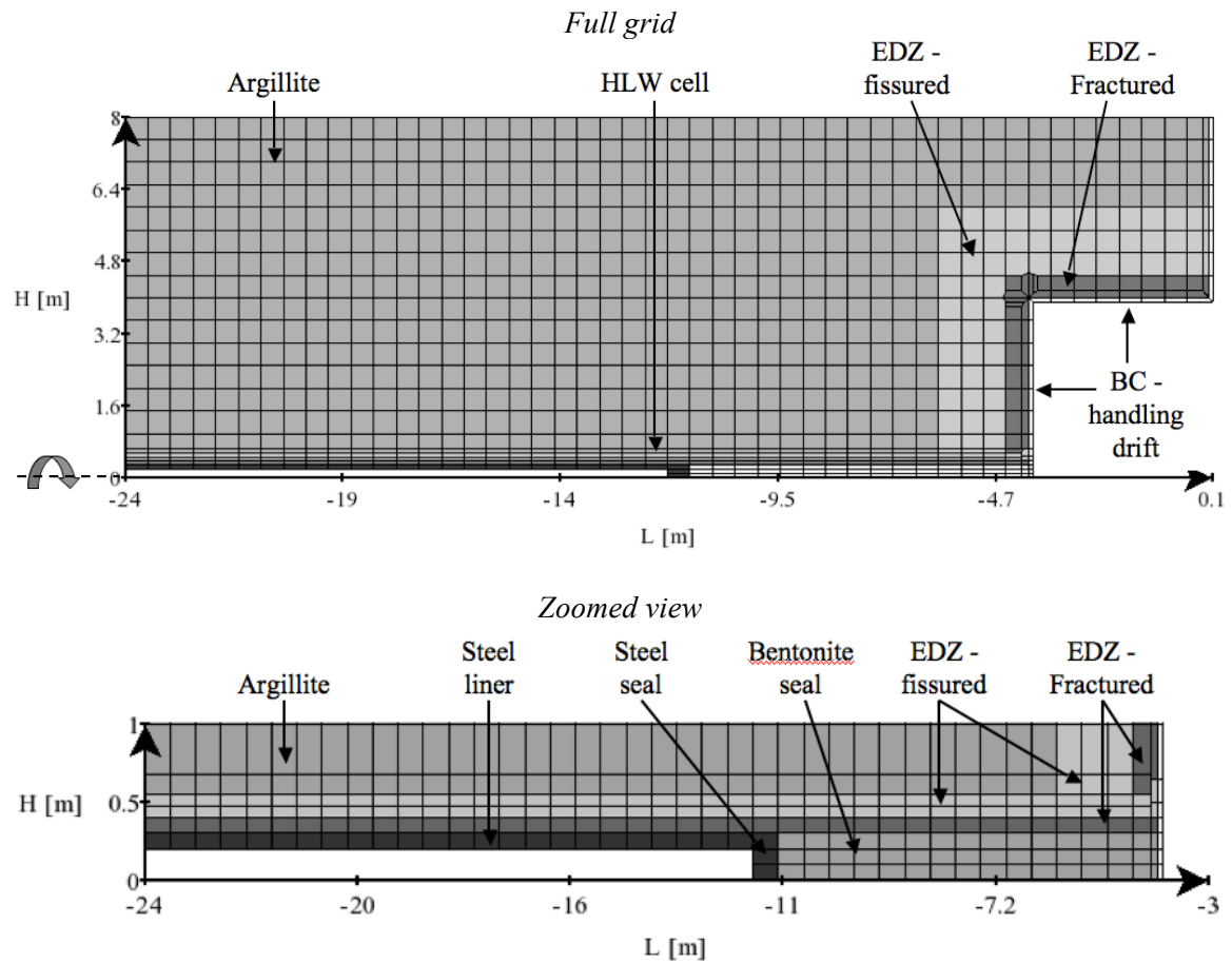
Figure 4. HLW disposal cell: 2D-cylindrical modeling grid (rotation around the length axis L); BC stands for boundary conditions, EDZ for the excavated damaged zone of the handling drift and the disposal cell.
