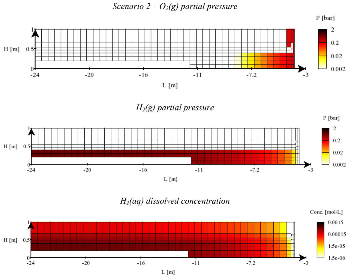
Figure 9. HLW disposal cell: 2D-profiles of oxygen and hydrogen partial pressures and of dissolved hydrogen concentration, calculated after 100 y for scenario 2.
