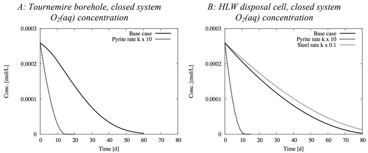
Figure 2. Dissolved oxygen consumption under water-saturation scenario 1b, i.e. a closed system without air ventilation, calculated at the back of the Tournemire borehole (-9.25, 0.02 m) and the middle of the HLW disposal cell (-15.25, 0.35 m); sensitivity analysis on the rate constant of pyrite oxidation and steel oxalic corrosion.
