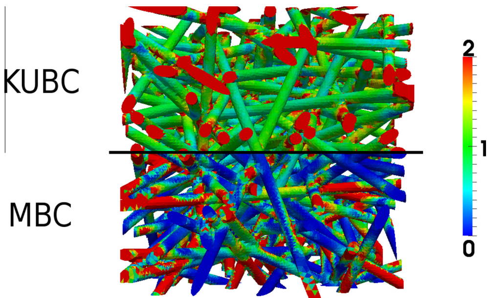
Fig. 12. \frac{\sigma_{zz}}{V_f(\sigma_{zz})} mapping for a V = 50^3 realization under hydrostatic load using KUBC (top) and MBC (bottom).
