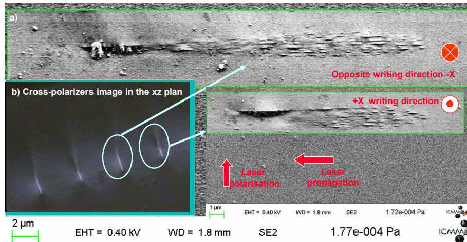
Fig. 1. FEG-SEM, Secondary electrons images of the cross-section of laser tracks written in opposite orientation. The laser parameters were: 0.4 \mu\text{J}/\text{pulse} , 800 nm, 160 fs, 200 kHz, 0.5 NA, 100 \mu\text{m}/\text{s} i.e. 2 \cdot 10^3 pulses/ \mu\text{m} . (b) Cross-section microscope images taken between crossed polarizers with the birefringent lines slow axis oriented at about 30^\circ of the polarizer.
