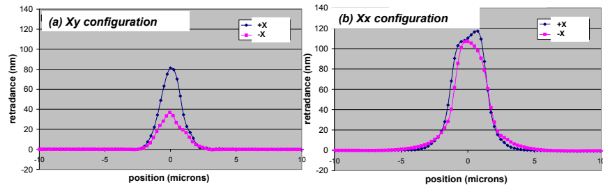
Fig. 3. Plot of the retardance profile with respect to writing velocity in left-to-right (+ X) direction (blue squares) and right-to-left (-X) direction (pink squares). (a) Perpendicular configuration quoted Xy, (b) parallel configuration quoted Xx. The laser parameters were: 0.4 \mu\text{J/pulse} , 800 nm, 160 fs, 200 kHz, 0.5 NA, 100 \mu\text{m/s} i.e. 2 \cdot 10^3 pulses/ \mu\text{m} .
