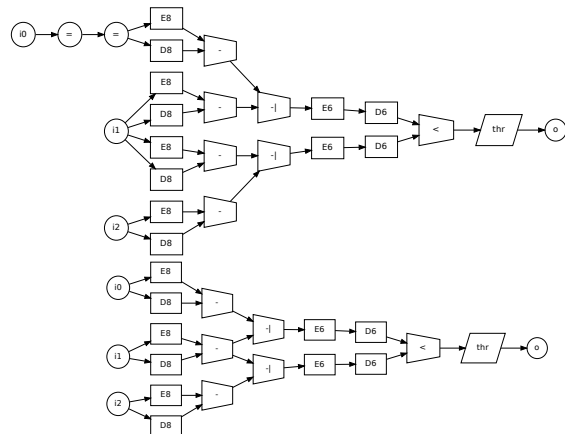
Figure 11. Initial and optimized DAG from application OOP
