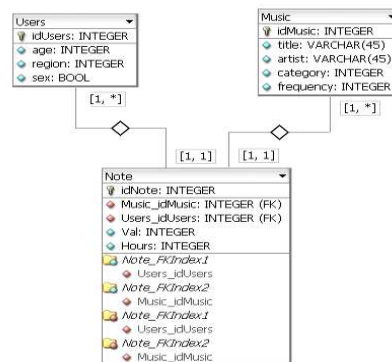
Figure 2: Data base.
