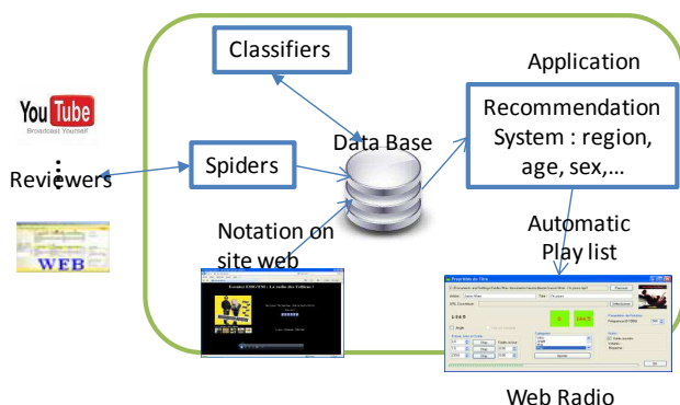
Figure 1: Application architecture.
