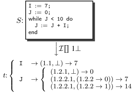
Figure 1. Syntax and semantics for an Imp program: (k, t) = \mathcal{T}[S]1\perp .
