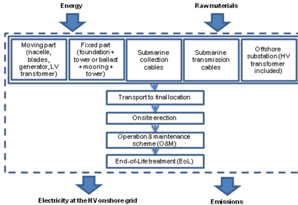
Fig. 2. Components considered for the offshore modular LCA model
