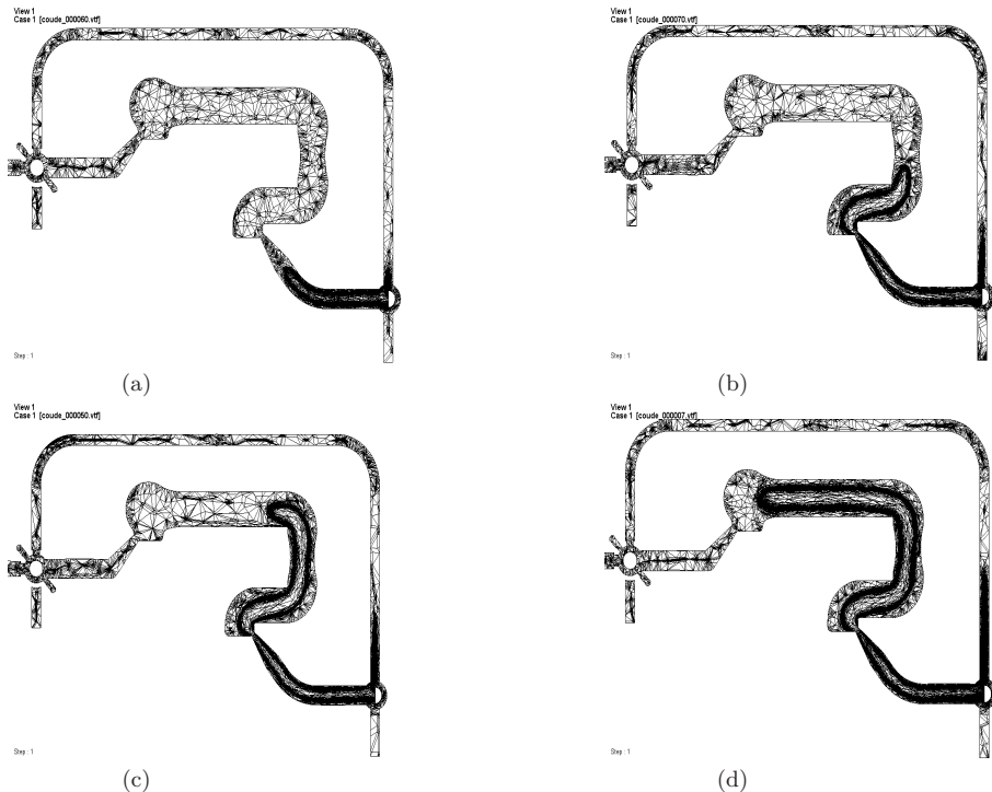
Fig. 11. Evolution of water/polymer fronts during the water assisted injection process
