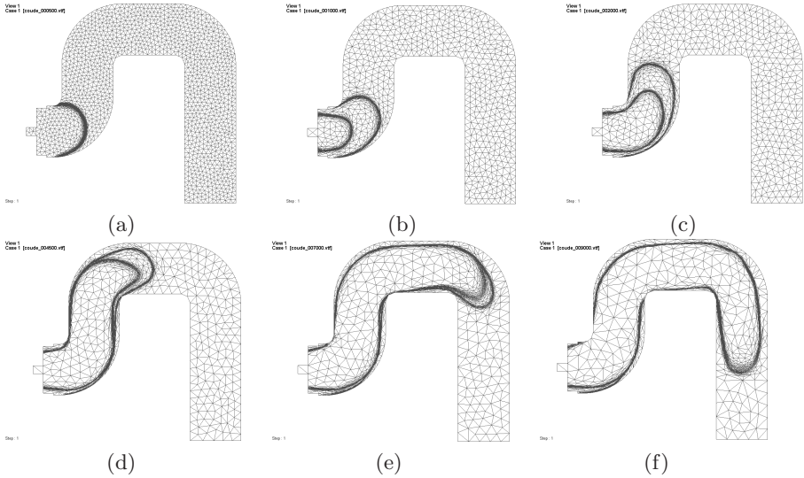
Fig. 8. Evolution of the polymer/air and water/polymer fronts during the water assisted injection process
