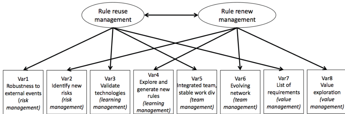
Figure 1: measurement model
