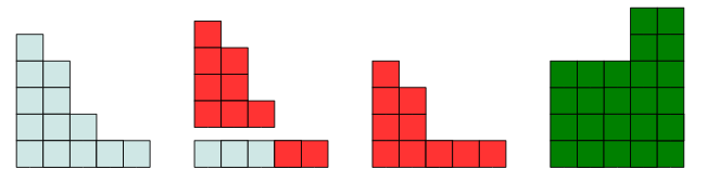
Figure 7 Ultimate Opening with \Delta=1 . From left to right: profile I , differences between openings, R_\theta and q_\theta
