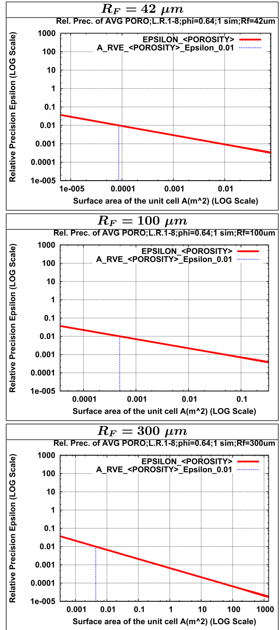
FIG. 10. Evolution of the relative precision of estimation \epsilon of \langle \Phi \rangle over the surface area A of one random realization ( n=1 ) at different scales ( R_F = 42 \mu m, 100 \mu m, and 300 \mu m ). The minimum surface area A on the Ox axis is equal to A_C in Table I. Blue dashed vertical line: \epsilon = 1 \% . Logarithmic scales.
