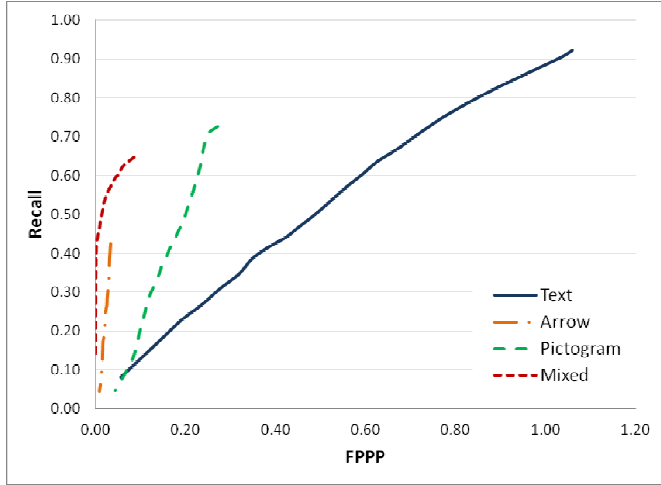
Figure 10. Frame-by-frame evaluation of our complete detection + recognition chain: \text{Recall} = f(\text{False Positive Per Positive}) curves separately for each meta-class.
