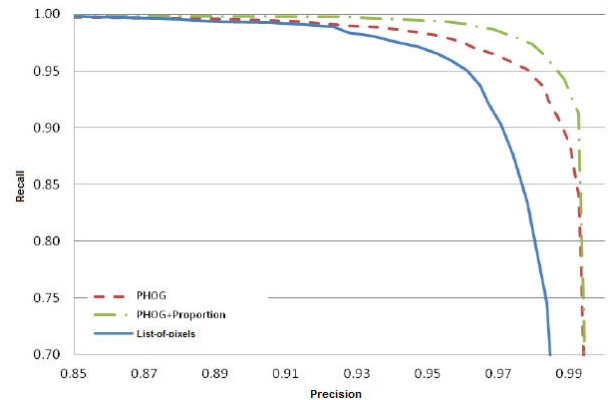
Figure 7. Comparison of classification performance of 3 descriptors: pixels of rescaled image (bottom curve, in blue), pHoG (middle in dashed red), and pHoG-Dp (top curve, in green dash-point).
